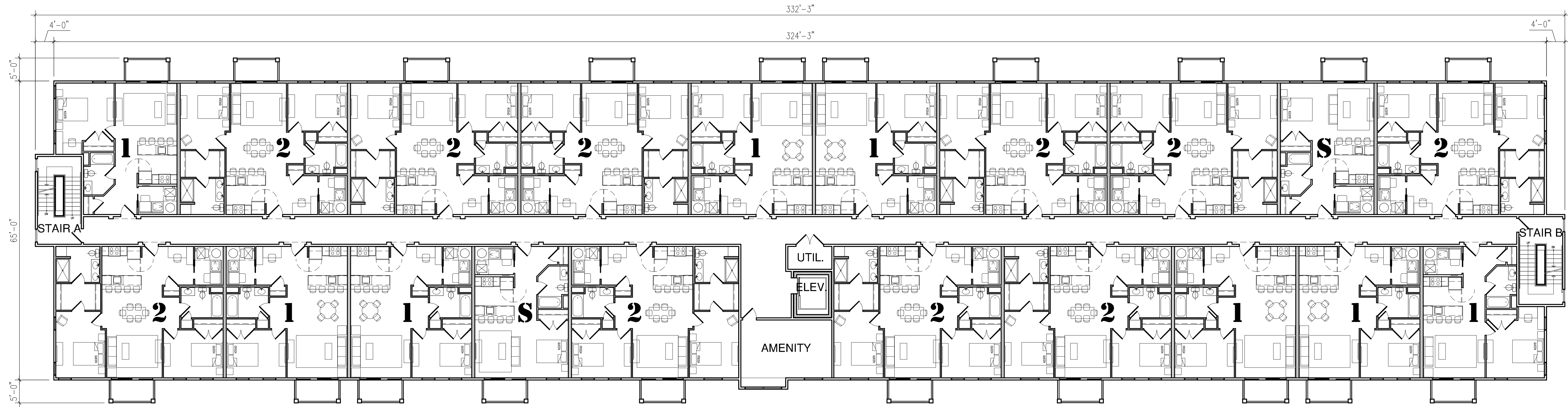
② TYPICAL UPPER FLOOR PLAN 3/32" = 1'-0"
